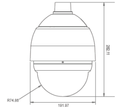
Dimension IB-HD82PTZ
