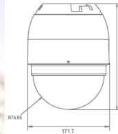
Dimension IB-HD72PTZ
